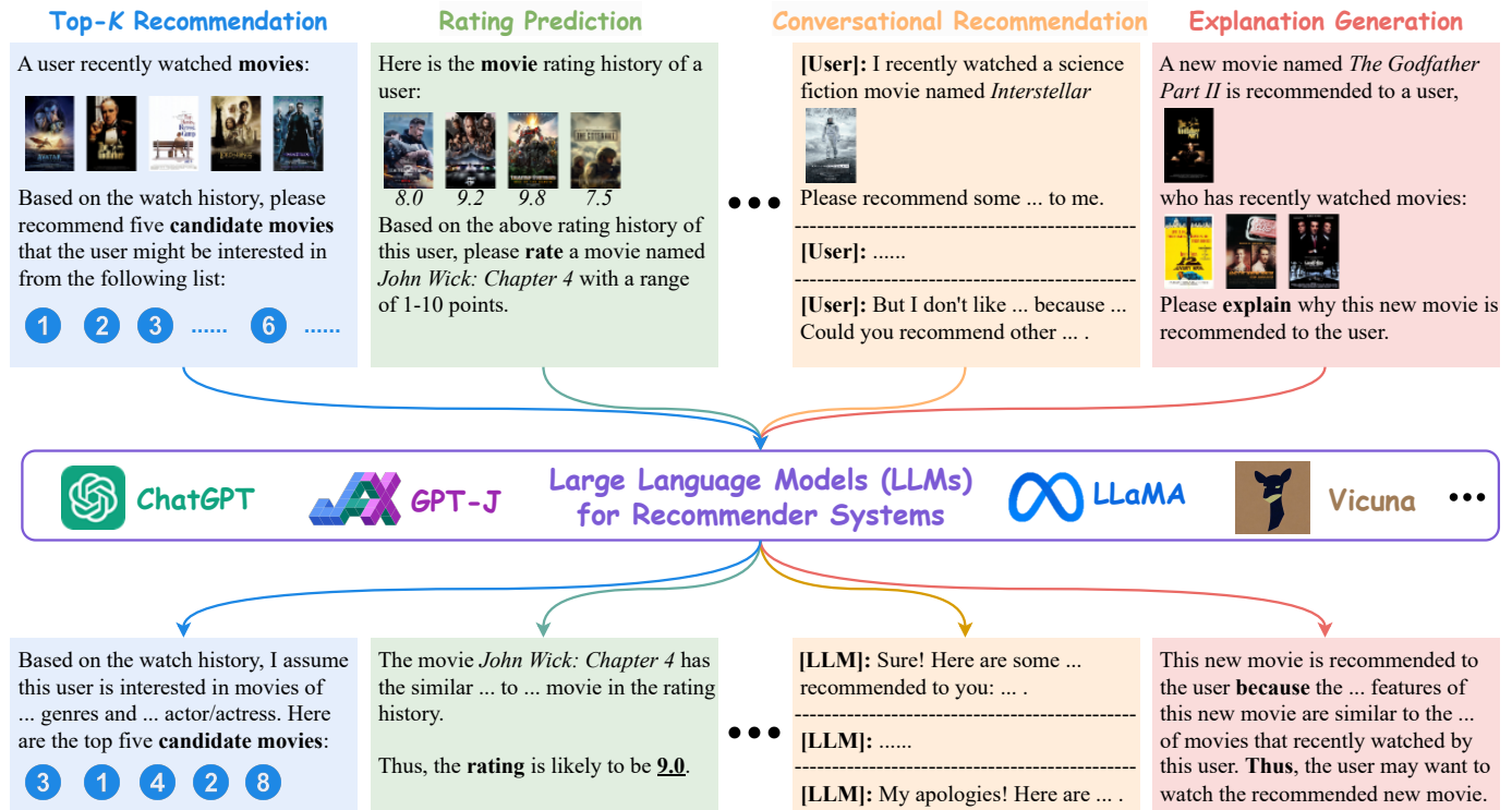
Figure 1: Examples of the applications of LLMs for various recommendation tasks in the scenario of movie recommendations. LLMs can leverage textual data (or even multimodal data like images) for recommendation tasks.
